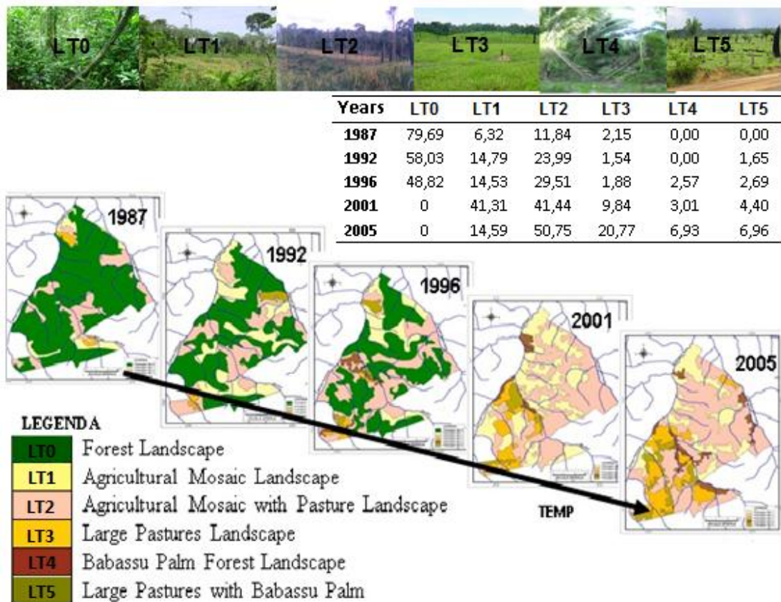
Figure 3. Dynamics of landscape types in SP-Benfica, southeastern of Pará State, Itupiranga municipality, Brazil.
