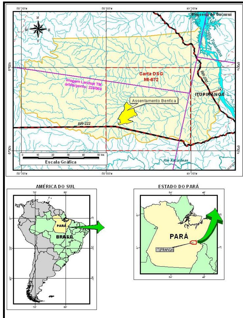
Figure 1. Location of the area of SP-Benfica, southeastern of Pará State, Itupiranga municipality, Brazil.
